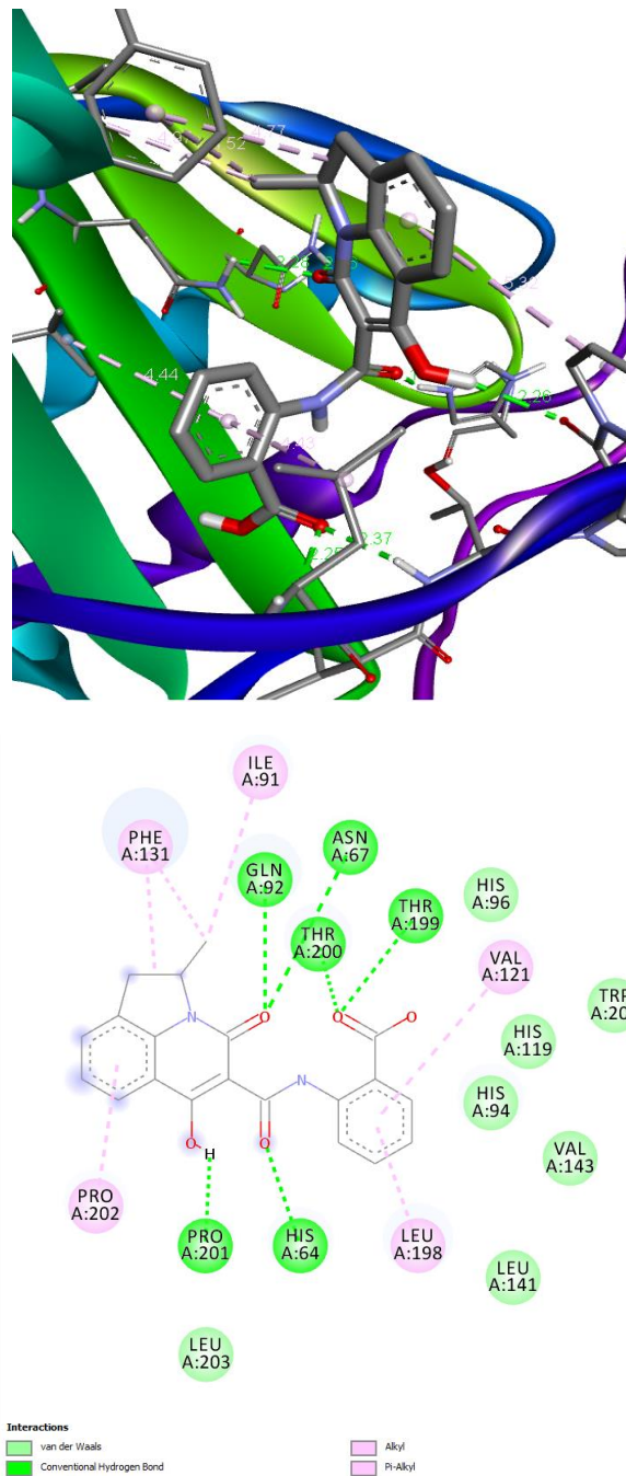
Fig 5. The molecule Ia superposition and the diagram of intermolecular interactions in the complex with the carbonic anhydrase II PDB ID: 1Z9Y
