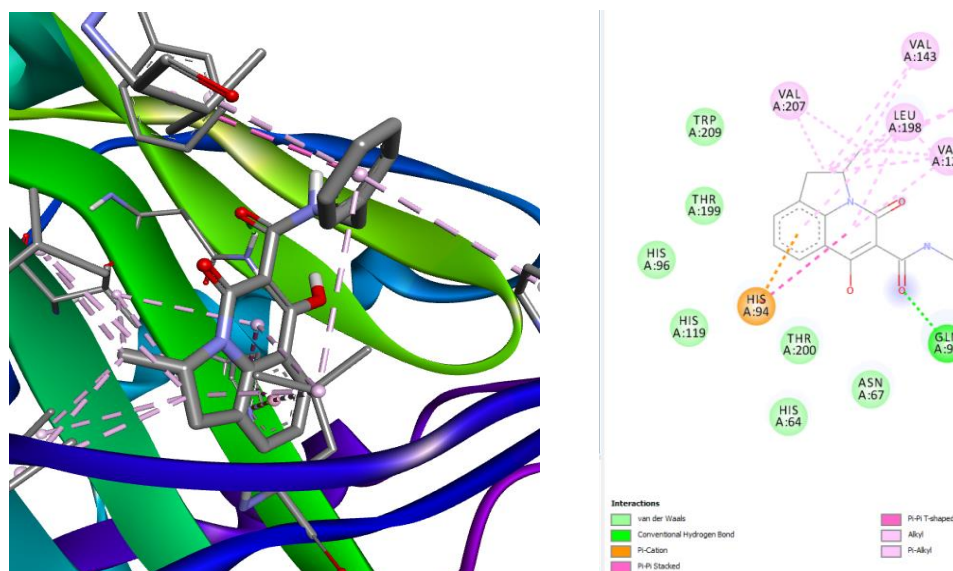
Fig 6. The molecule 1b superposition and the diagram of intermolecular interactions in the complex with the carbonic anhydrase II PDB ID: 1Z9Y
