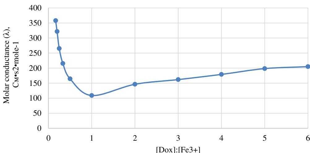
Fig. 4. Dependence of molar conductivity on the ratio of molar concentrations [\text{Dox}]:[\text{Fe}^{3+}] dissolved in water at a temperature of 295 K
