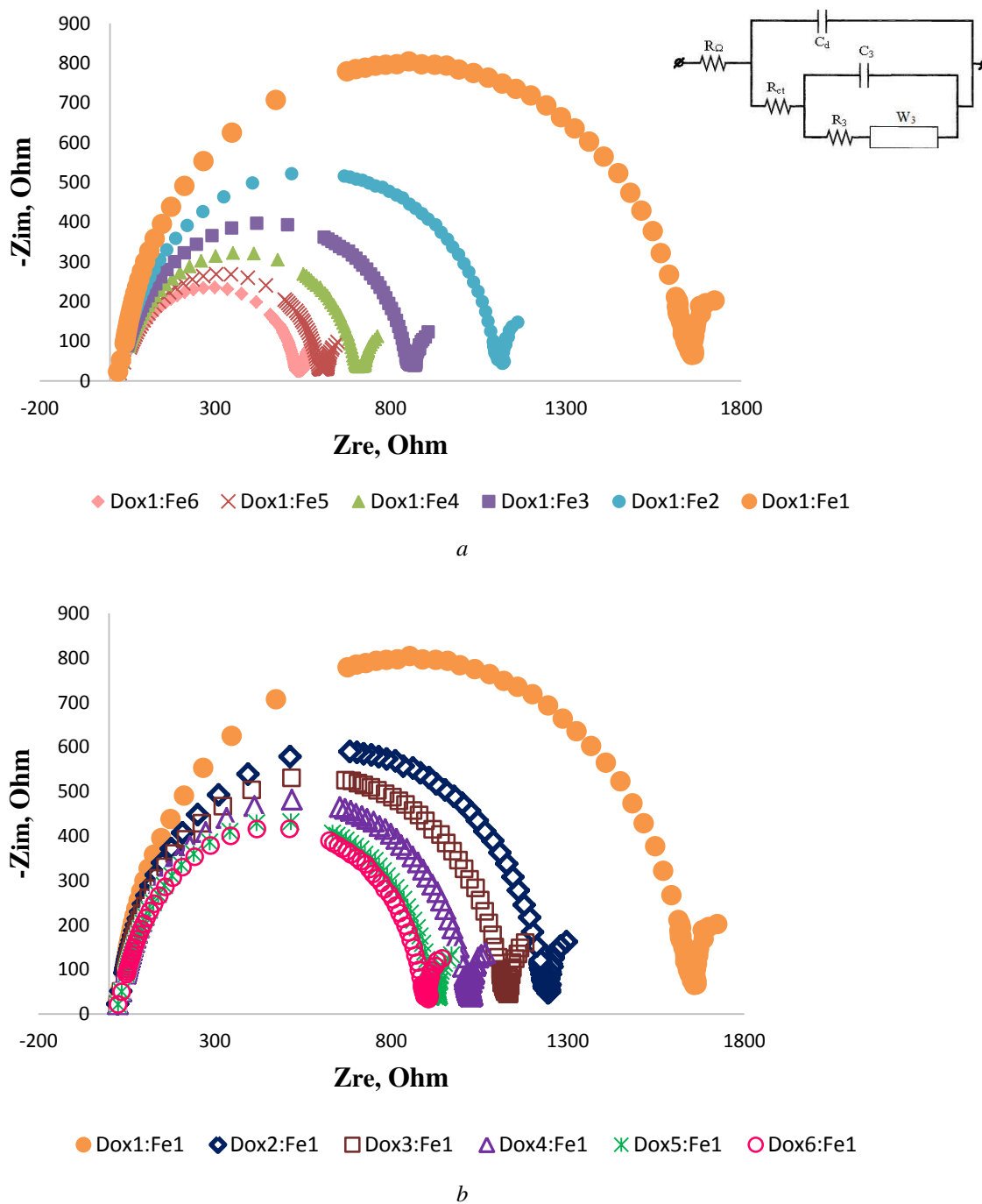
Fig. 3. Nyquist curves for doxycycline and iron (III) chloride solutions in different concentration ratios, measured at a temperature of 295 K: a – increase in Fe^{3+} concentration; b – increase in doxycycline concentration
