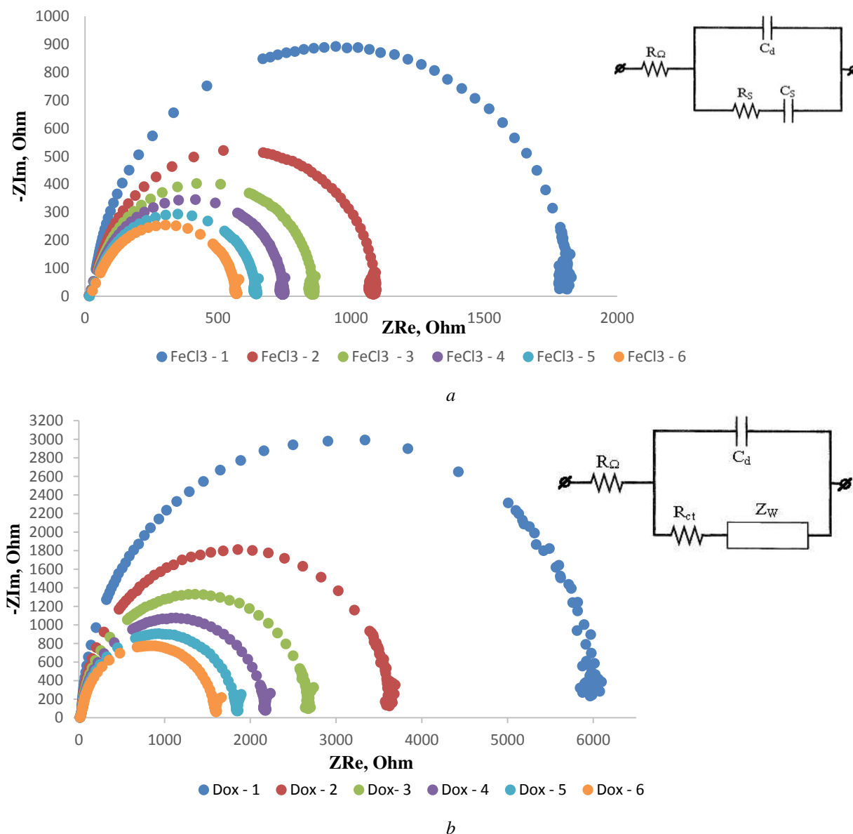
Fig. 2. Nyquist curves with inset of equivalent electrical circuit of the measuring cell for 6 molar concentrations of solutions of a – FeCl 3 ; b – doxycycline hyclate
