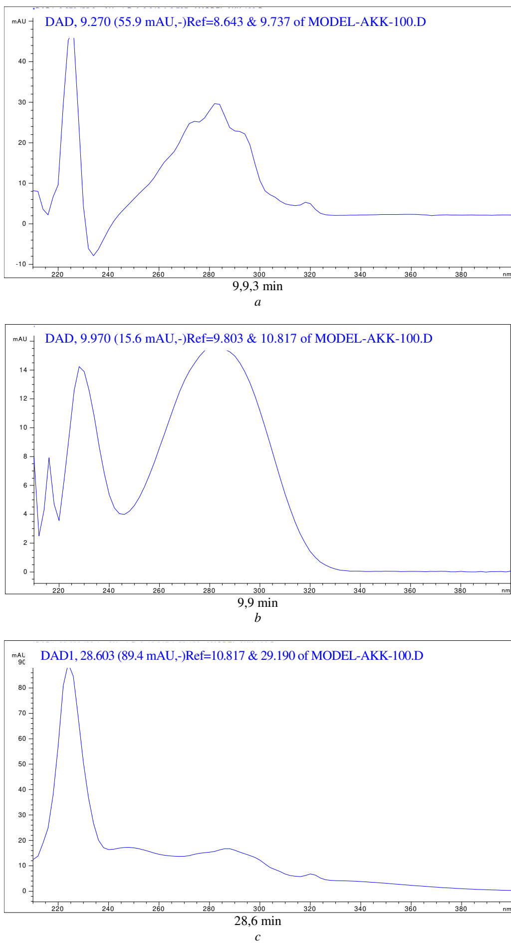
Fig. 3. UV spectra: a – dansyl chloride; b – para-aminobenzoic acid; c – aminocaproic acid derivative
