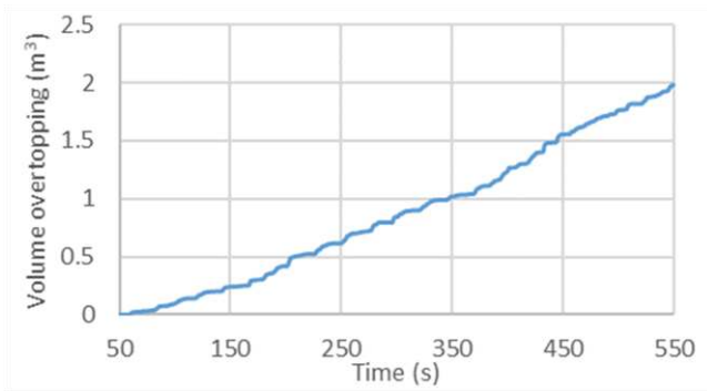
Gambar 4.4 Grafik kumulatif volume overtopping Model B1.60
