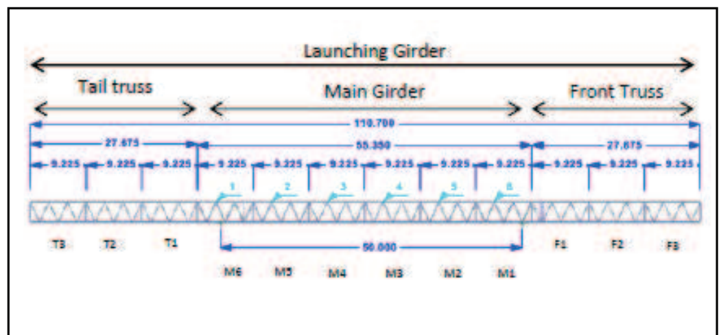
Figure 1: Launching girder.
