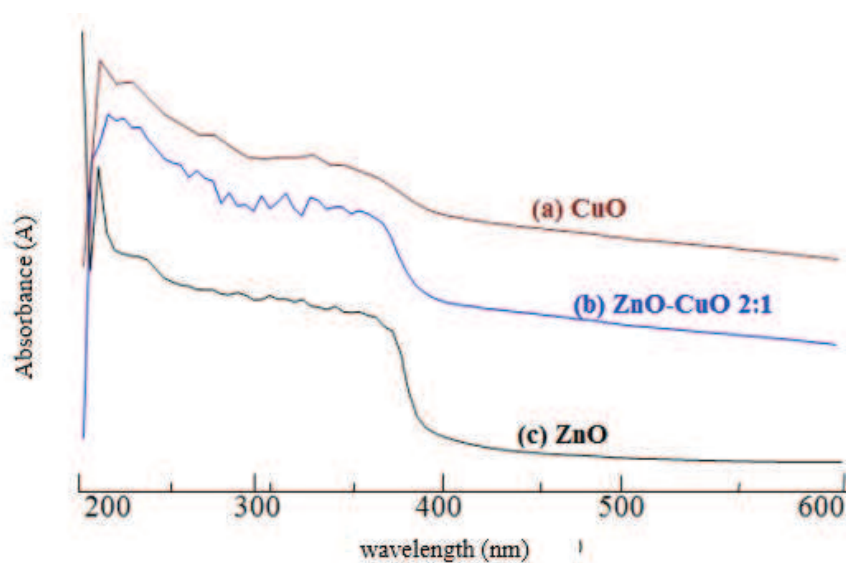
Figure 3: Spectral Absorbance of (a) CuO, (b) ZnO-CuO 2: 1 and ZnO Catalysts from UV-DRS Spectrophotometers.
