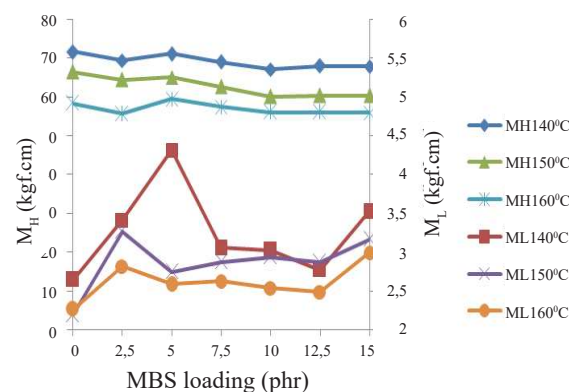
Figure 2. M_H and M_L of the NR/NBR/MBS blends.
