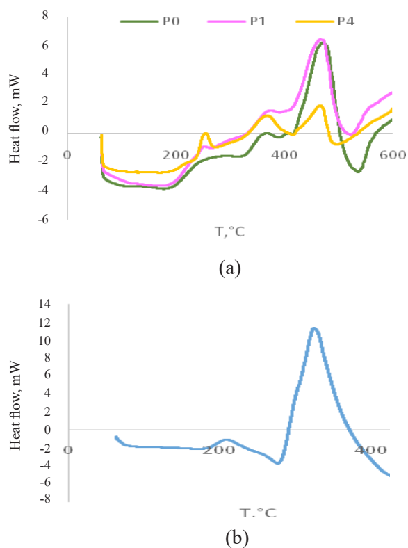
Figure 8. DSC curve of (a) MBS and (b) NR/NBR blends.
