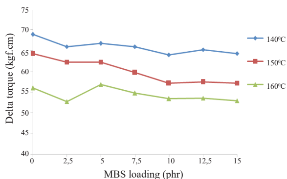
Figure 3. The delta torque of the NR/NBR/MBS blends at 140, 150 and 160 °C.
