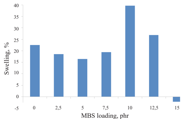
Figure 6. Swelling percentages of NR/NBR/MBS blends.
