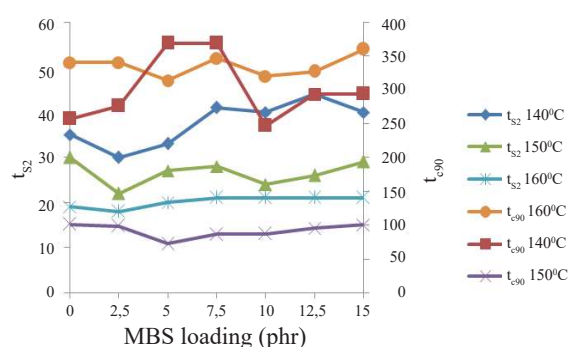
Figure 1. t_{s2} and t_{c90} of the NR/NBR/MBS blends.
