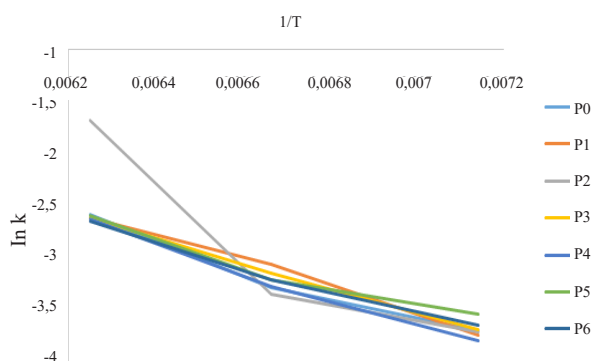
Figure 4. The Arrhenius plot for NR/NBR/MBS blends obtained from the rheographs.
