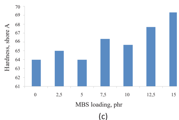
Figure 5. Mechanical properties of NR/NBR/MBS blends: (a) tensile strength, (b) elongation, (c) hardness.
