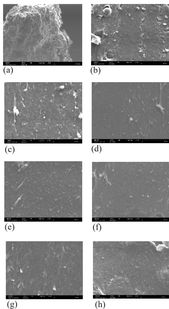
Figure 7. SEM micrographs of the tensile fracture surface of 50/50 (w/w) of NR/NBR blends (a) MBS 500x (b) without MBS 1000x (c) 2.5 phr MBS 1000x (d) 5 phr MBS 1000x (e) 7.5 phr MBS 1000x (f) 10 phr MBS 1000x (g) 12.5 phr MBS 1000x and (h) 15 phr MBS 1000x.
