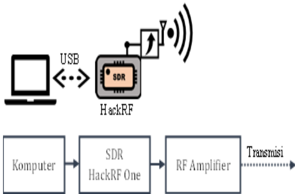
Gambar 5. Blok diagram transmitter.
