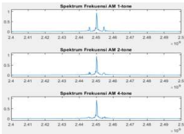
Gambar 9. Plot MATLAB sinyal AM domain frekuensi setiap tone.
