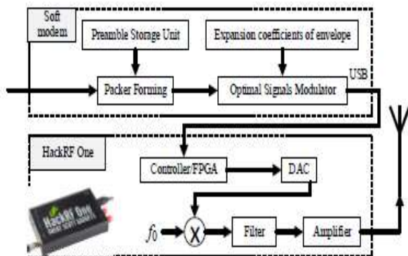
Gambar 3.Diagram blok SDR HackRF One.
