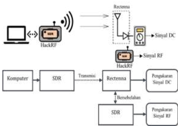
Gambar 2. Diagram blok sistem WPT penelitian.
