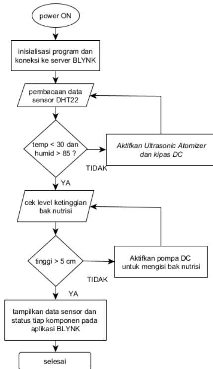
Gambar 12. Flowchart algoritma program.
