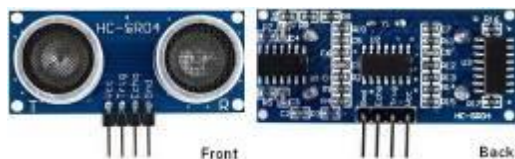
Gambar 7. Modul sensor HC-SR04.
