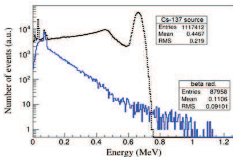
Figure 5: Energy spectrum distribution of beta radiation from Cs-137 source for \text{CaMoO}_4 detector.
