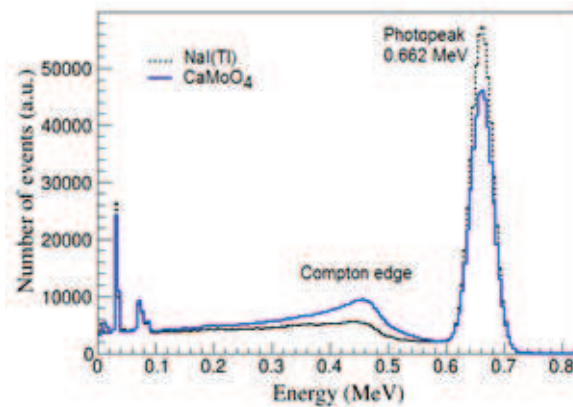
Figure 3: Energy spectrum distribution of Cs-137 detected by NaI(Tl) and \text{CaMoO}_4 .
