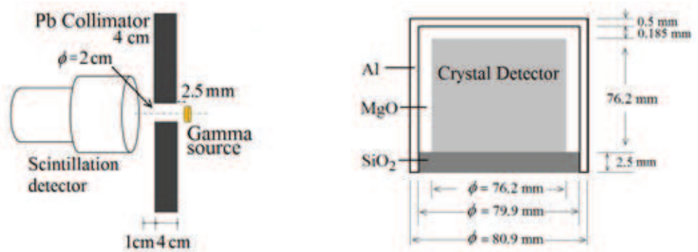
Figure 1: Schematic design of detector and simulation geometry construction.
