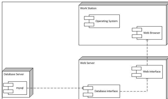
Gambar 17. Deployment Diagram
