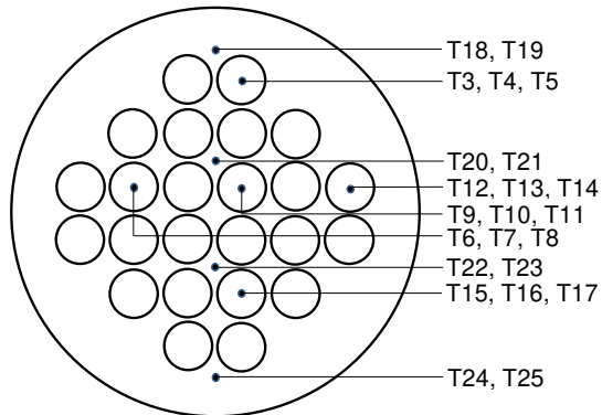
Figure 2. Capsule Arrangement
