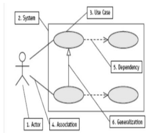
Gambar 3. Elemen Use Case Diagram
