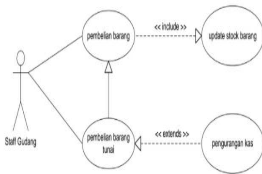
Gambar 4. Contoh Use Case Diagram
