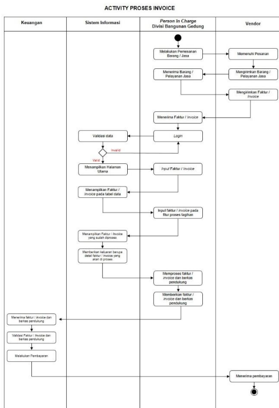
Gambar 6. Activity Diagram
