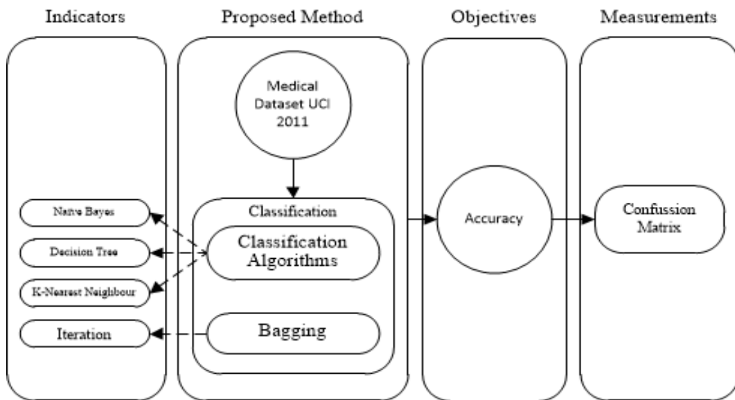
Gambar 1. Metode Penelitian
