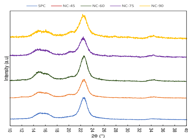
Figure 2. XRD diffractogram of sugar palm cellulose (SPC) and sugar palm cellulose nanocrystal at various hydrolysis times (NC-45, -60, -75, -90)
