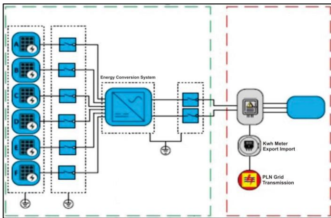
Figure 3. Rooftop PV Plant network topology on-grid system
