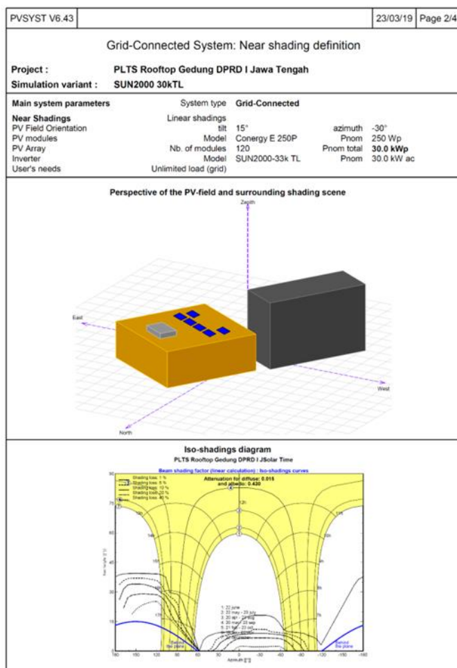
Figure 10. Shadow analysis simulation results using PVSyst 6.4.3. software
