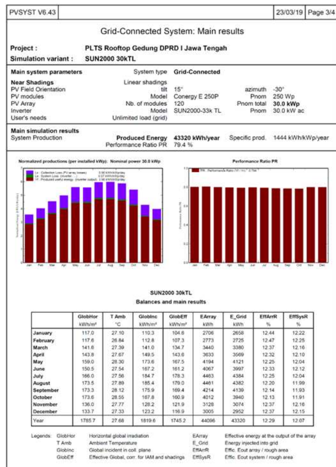
Figure 11. Performance ratio simulation results using PVSyst 6.4.3. software
