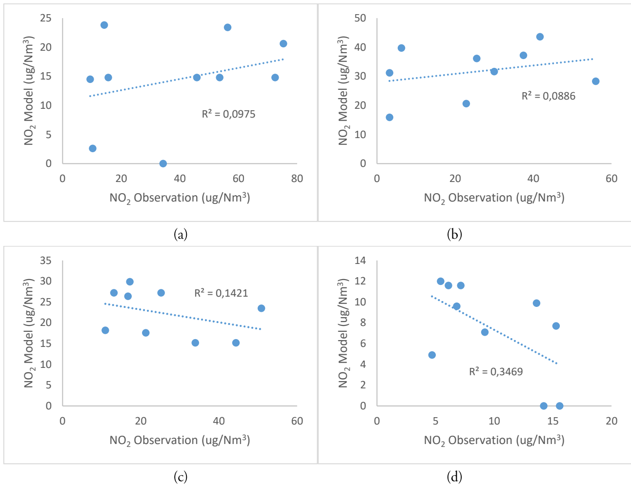
Figure 6. Scatter plot showing the relationship between \text{NO}_2 observation and model; (a) 1 st quarter, (b) 2 nd quarter, (c) 3 rd quarter, (d) 4 th quarter
