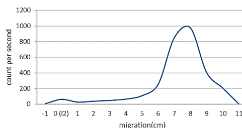
Figure. 2 Radiochromatogram of ^{131}\text{I} -Rutin
