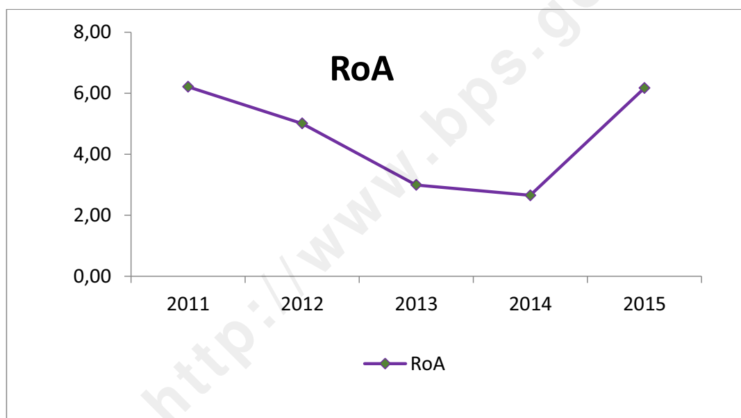
Gambar 5.3 Return on Assets (RoA) Perusahaan Telekomunikasi di Indonesia, 2011 – 2015 Figure 5.3 Return on Assets (RoA) of Telecommunication Companies in Indonesia, 2011 – 2015
