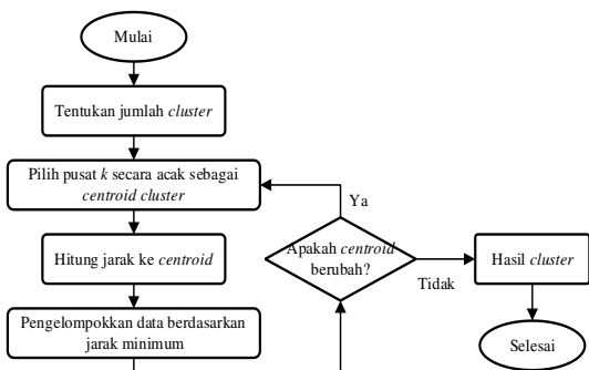
Gambar 3. Flowchart algoritma k-means clustering
