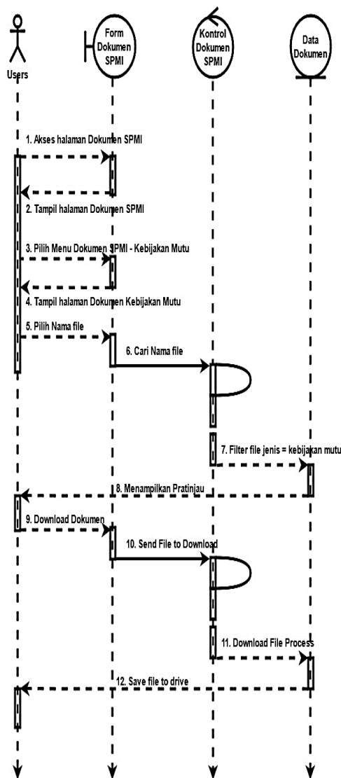
Gambar 4. Sequence diagram pratinjau dokumen SPMI
