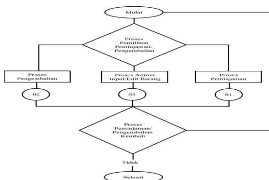
Gambar 2. Flowchart 1
