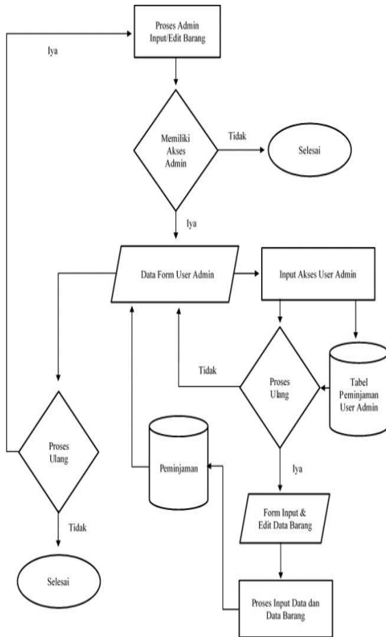
Gambar 4. Flowchart 3
