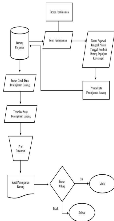
Gambar 3. Flowchart 2
