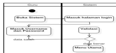
Gambar 3.3 Activity Diagram Login
