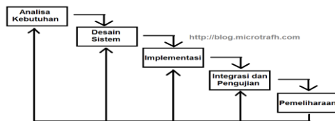
Gambar 3.1 Waterfall
