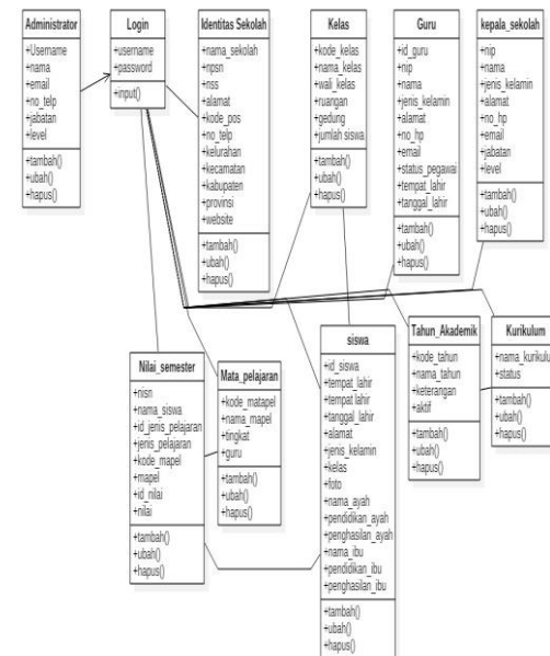
Gambar 3.8 Class Diagram Sistem Usulan
