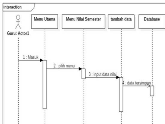
Gambar 3.6 Sequence Diagram Input Nilai
