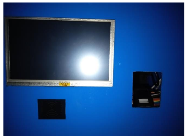
Gambar 3 Implementasi Prototype
