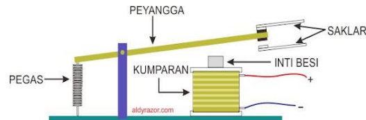
Gambar 2.12 Cara Kerja Relay
