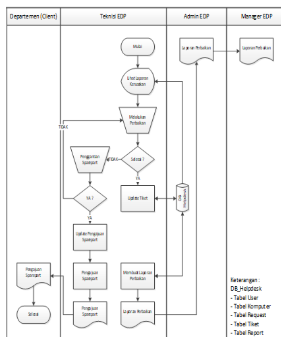
Gambar 2 Flow of Document Prosedur Penanganan Kerusakan
