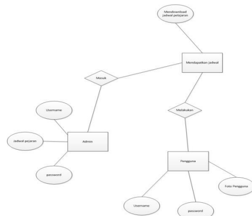
Gambar 3. Diagram ERD
