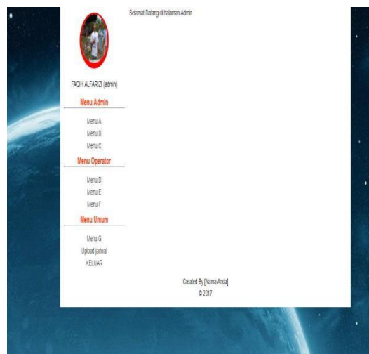
Gambar 7. Halaman Admin
