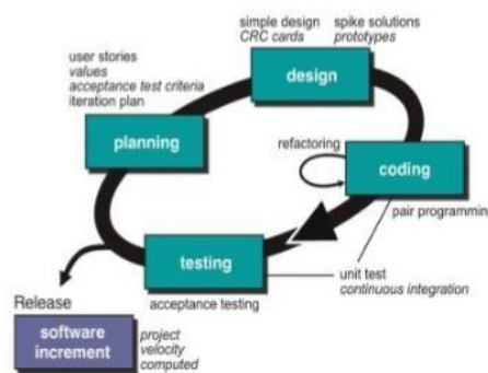
Gambar 1. Tahapan Extreme Programming
