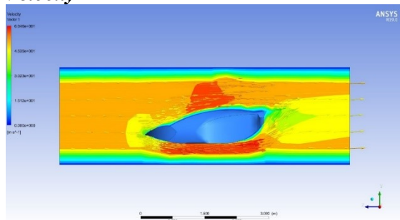
Gambar 12 Velocity Contour Streamine Model 3
