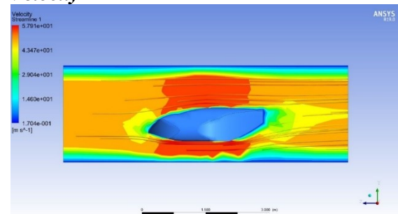
Gambar 8 Velocity Contour Streamline Model 2
