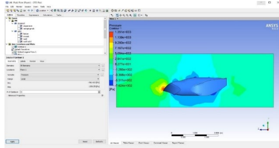
Gambar.10 Presure Contour Model 2
