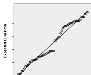
Gambar 2. Gambar P Plot dan Scater Plot
