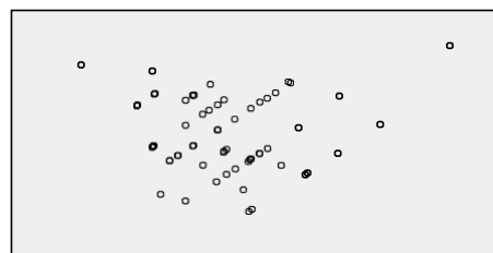
Gambar 2. Gambar P Plot dan Scater Plot
