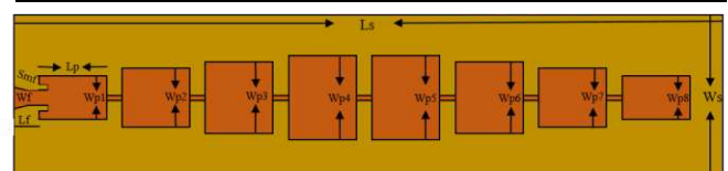
Gambar 5. Desain antenna fed series 1x8.
