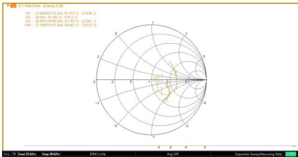
Gambar 10. Pengukuran impedansi antena fed series 1x8.
