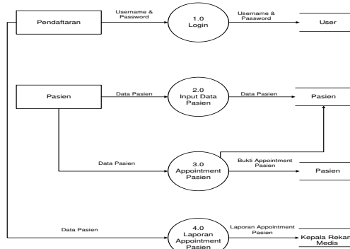
Gambar 6. DFD Level 0
