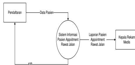
Gambar 5. Diagram Kontek
