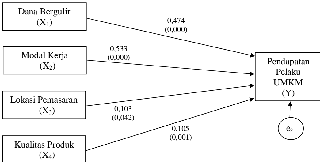
Gambar 2 Standardized Path Diagram Setelah Trimming
