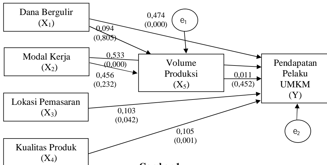
Gambar 1 Standardized Path Diagram
