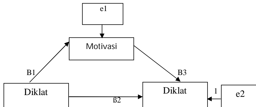
Gambar 3 Model Analisis Jalur (Path Analysis)
