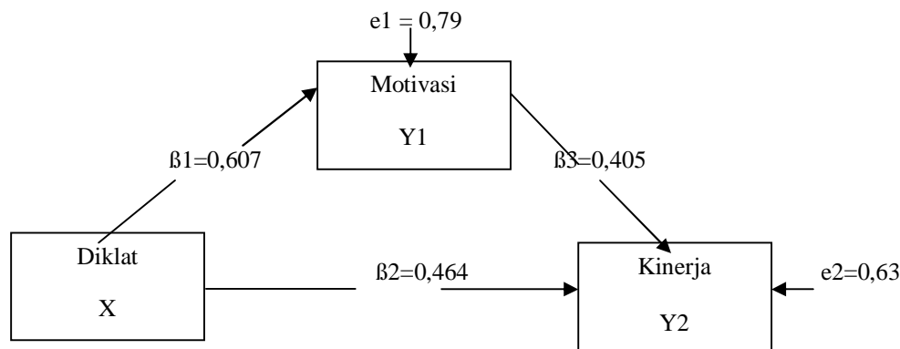
Gambar 4. Diagram Path Model Analisis
