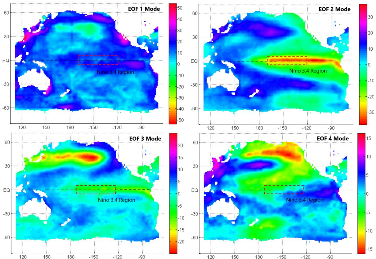
Figure 2. Plots of EOF-1, EOF-2, EOF-3, and EOF-4 mode spatial patterns based on Pacific Ocean surface temperature anomaly data.
