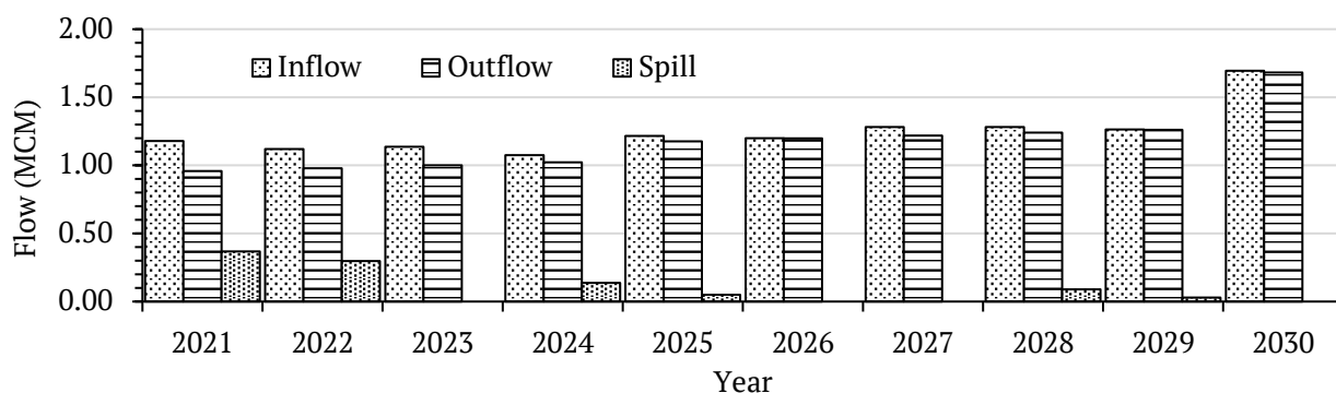
Figure 11. Beemos large reservoir Inflow-Outflow
