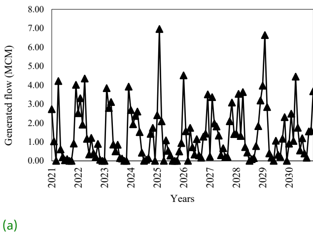
Figure 5. The monthly generated flow (a) Beemos; (b) Becora
