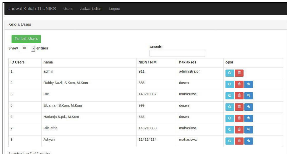
Gambar 9. Halaman User
