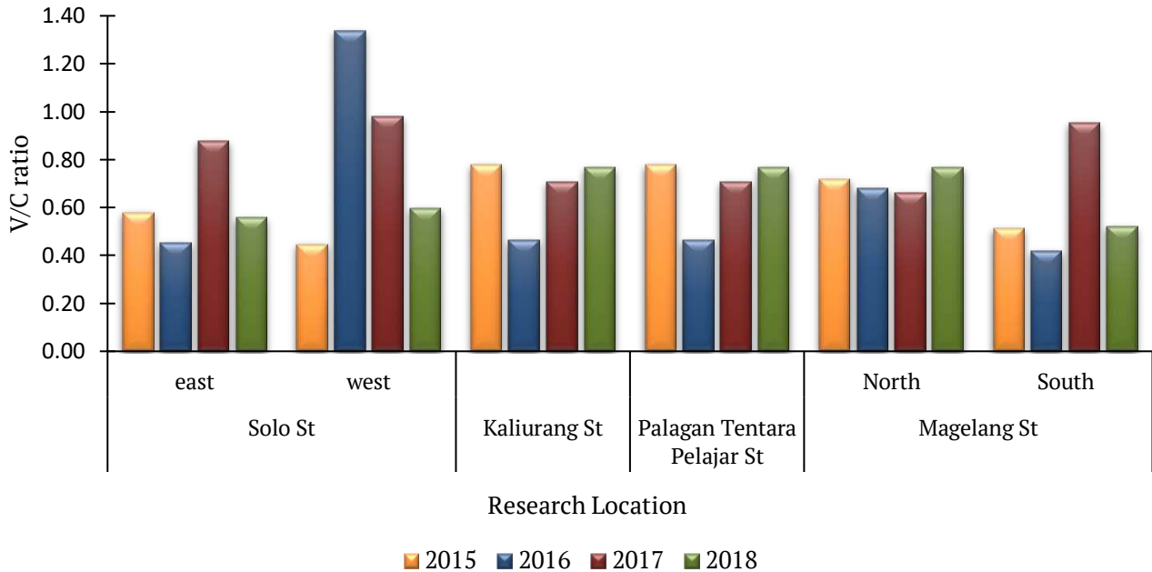
Figure 1: V/C Ratio in Some Arterial Roads in Yogyakarta from 2015-2018
