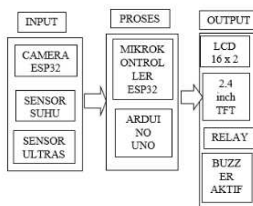
Gambar 5. Blok Diagram
