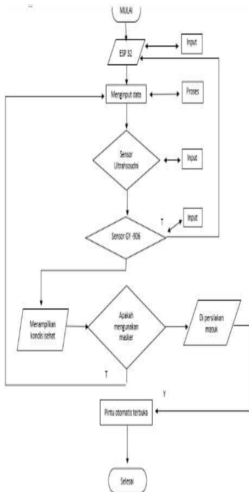
Gambar 6. Diagram Alir
