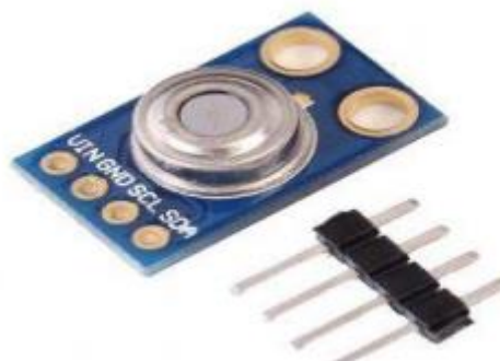
Gambar 2. Sensor GY-906 [5]
