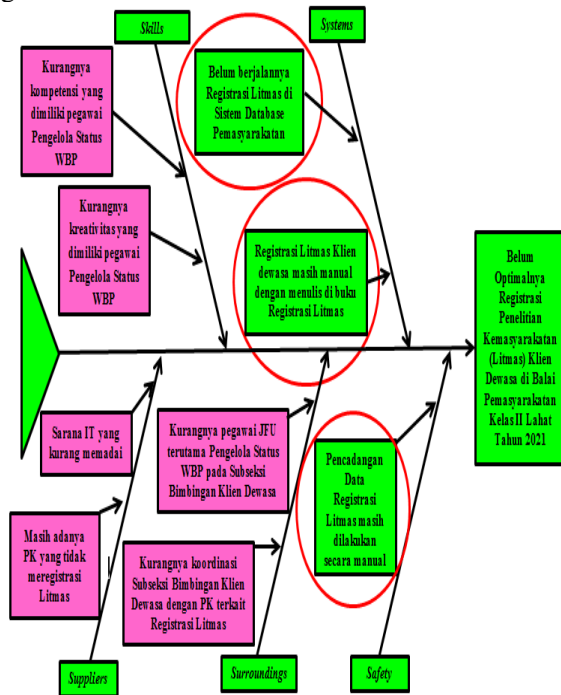
Gambar 1. Fishbone Diagram
