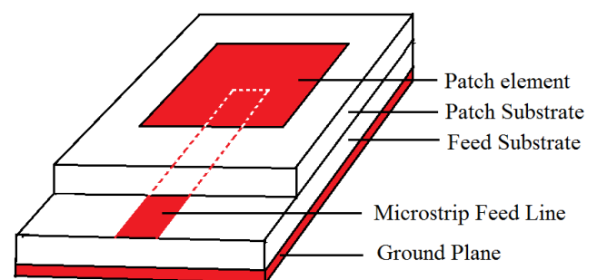
Gambar 4. Metode pencatutan proximity coupled feed .
