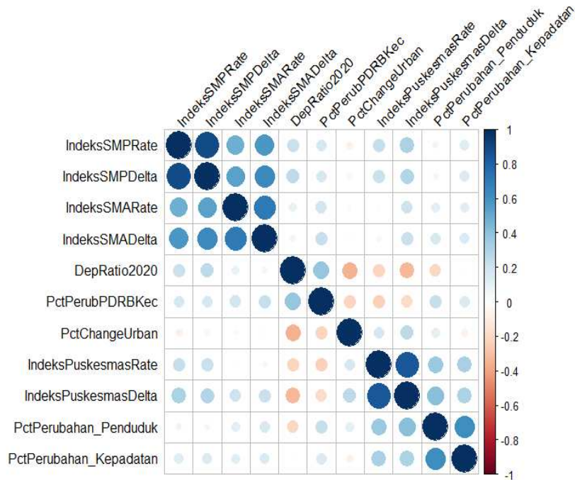
Figure 2. Correlation Plot
