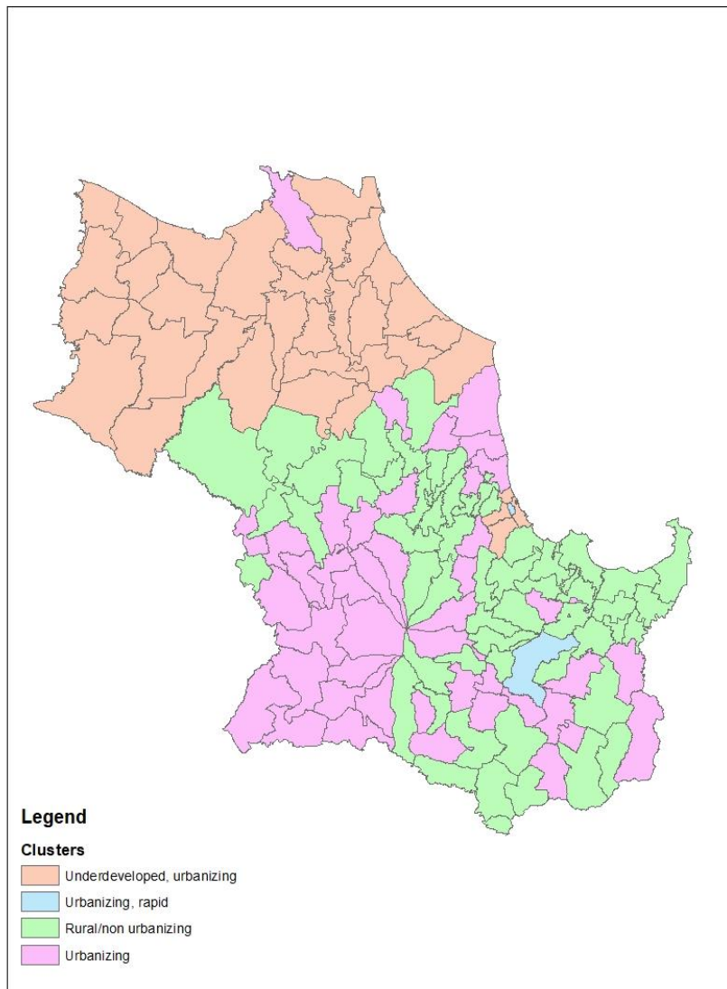
Figure 4. Clusters, mapped
