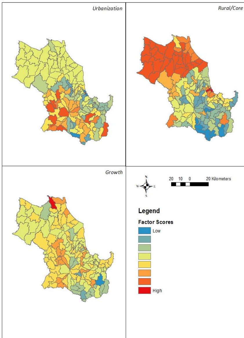
Figure 3. Factor Scores
