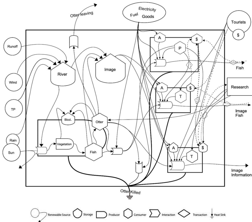
Figure 1. System diagram of the study area, the Aquidauana River, showing the connections within the ecosystem
