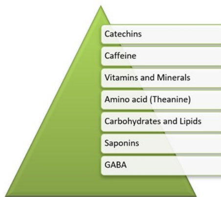
Figure 2. Chemical composition of green tea.
