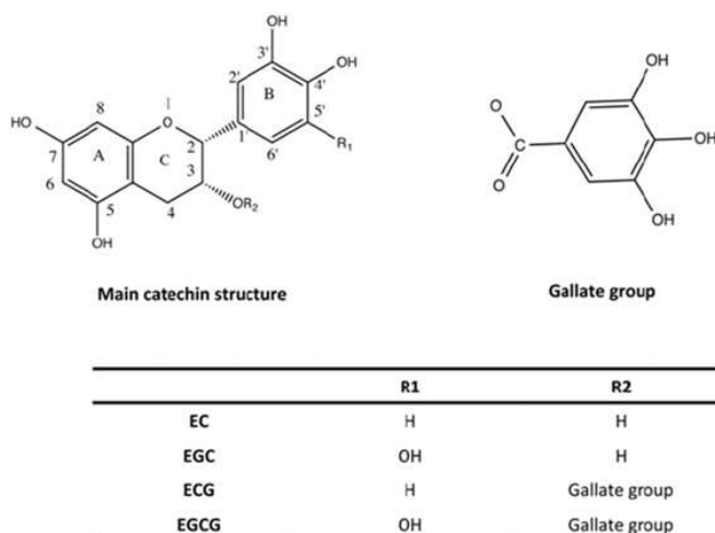
Figure 3. Different forms of Catechins.
