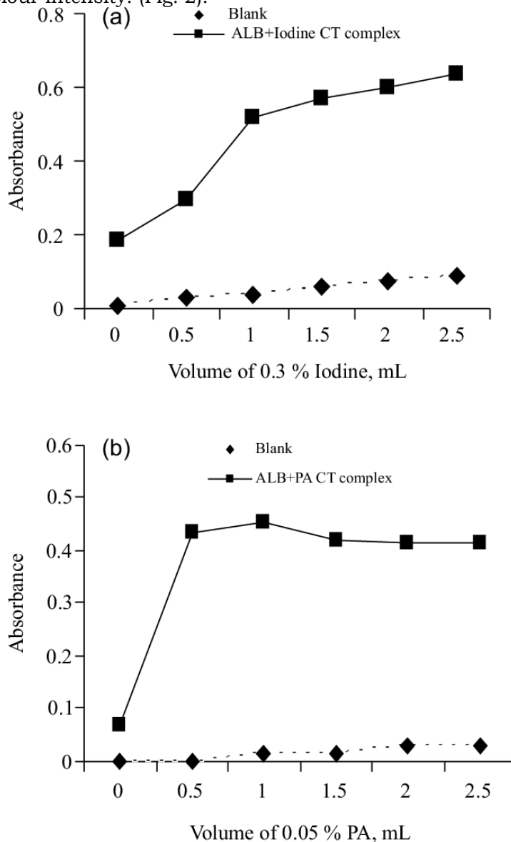
Figure 2. Impact of reagent concentration (a) ALB-iodine CT complex (-■-) [ 120 \mu\text{g mL}^{-1} ALB] and blank solution (-♦-); (b) ALB- picric acid CTcomplex (-■-) [ 30 \mu\text{g mL}^{-1} ALB] and blank solution (-♦-)
