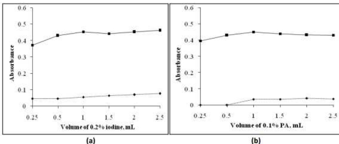
Figure 6. Impact of volume (a) 0.2% iodine in iodine method ( 10 \mu\text{g mL}^{-1}\text{ETN} ) (b) 0.1% picric acid in picric acid method ( 20 \mu\text{g mL}^{-1}\text{ETN} )
