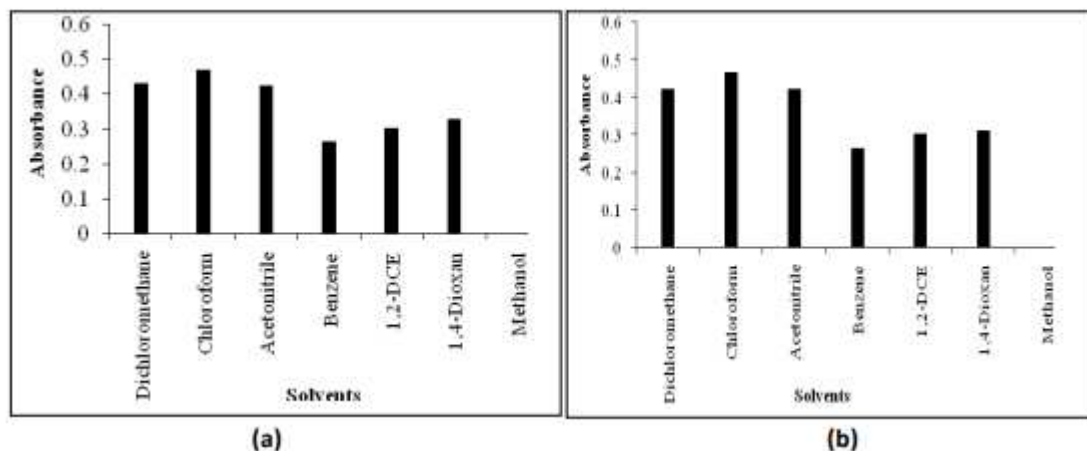
Figure 5. Impact of different solvents (a) ETN-iodine complex (■) [10 \mu\text{g mL}^{-1} ETN] (b) ETN-picric acid complex (■) [20 \mu\text{g mL}^{-1} ETN]
