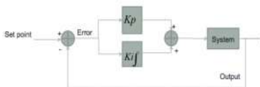
Figure: PI control loop
