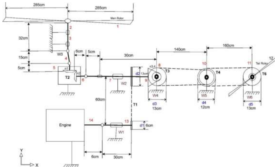
Figure 10: Kinematic diagram of the helicopter.
