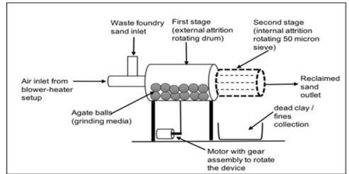
Fig. 2. Sieving and Attrition device [1]
