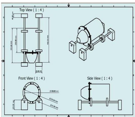
Fig.1. Schematic diagram of setup [3]
