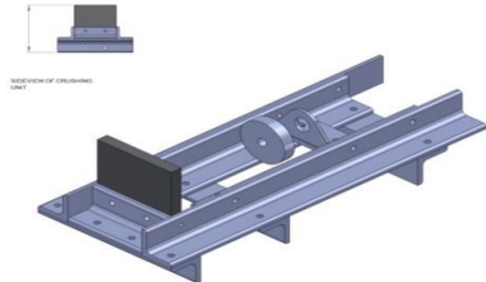
Fig. 16 Crushing Unit
