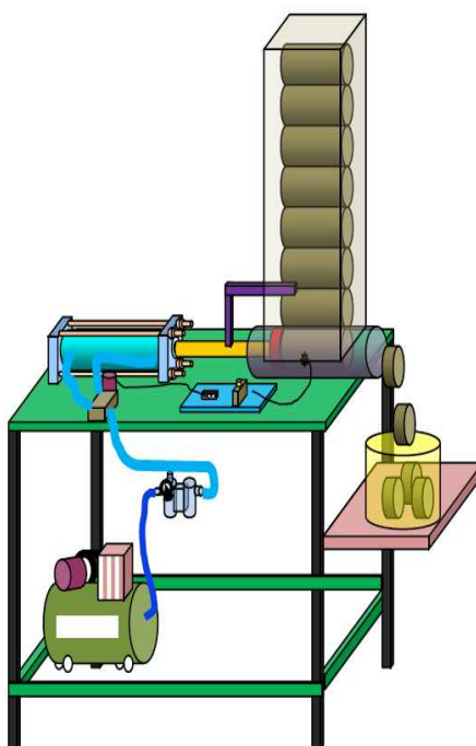
Fig. 1 Design of can crusher machine
