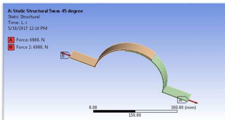
Figure 7. Applying boundary condition & equal forces on both sides
