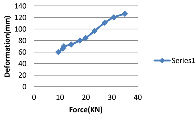
Graph2.2 6mm thickness both side weld
