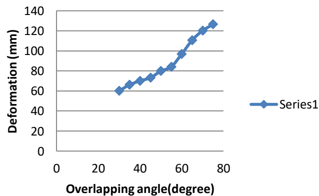
Graph 2.3 6mm thickness both side weld
