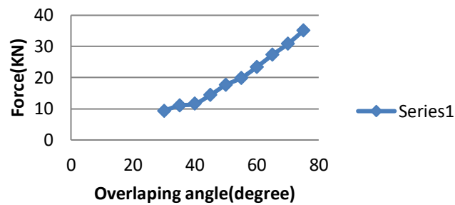
Graph2.1 6mm thickness both side weld
